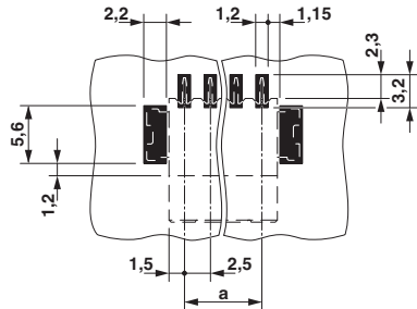
Drilling diagram
